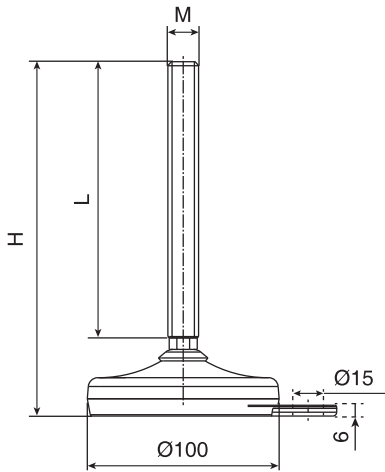
SS100 不锈钢底脚(带固定孔) SS100 STAINLESS STEEL FEET WITH FIXING HOLE
